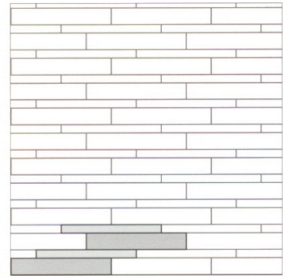
TS-6 33% /m² 5 x 60 cm / 2 x 24 inch 67% /m² 10 x 60 cm / 4 x 24 inch
